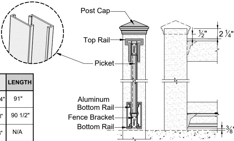
CUT VIEWS
