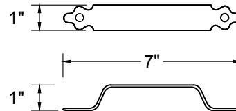
GATE HANDLE
