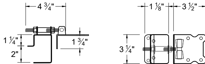
GATE HANDLE
