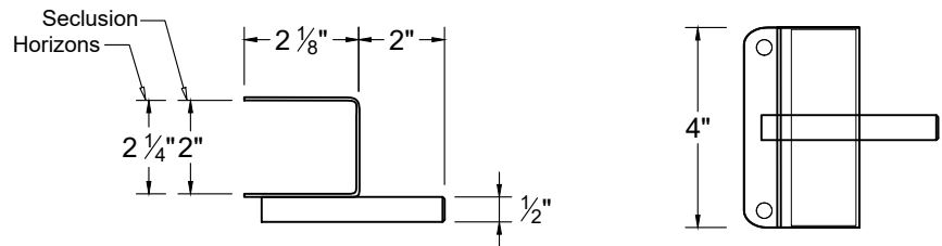
ADJUSTABLE HINGE
