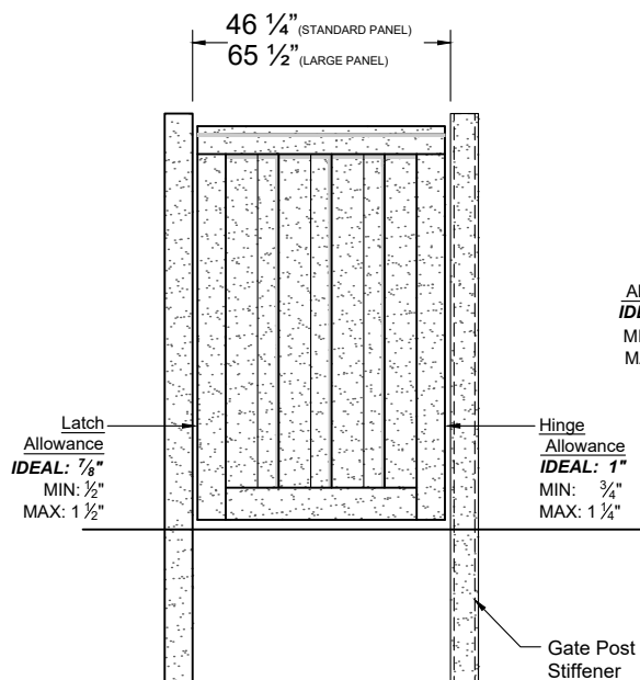
SINGLE GATE OPENING
