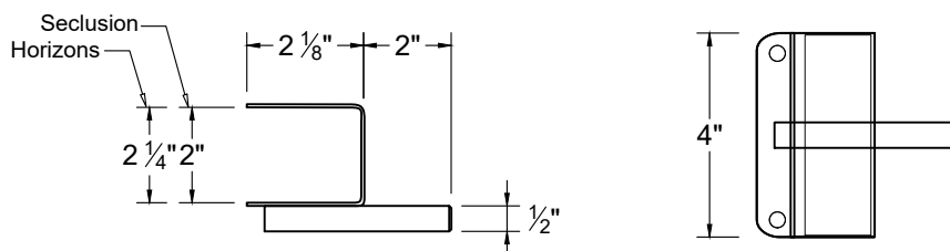
ADJUSTABLE HINGE
