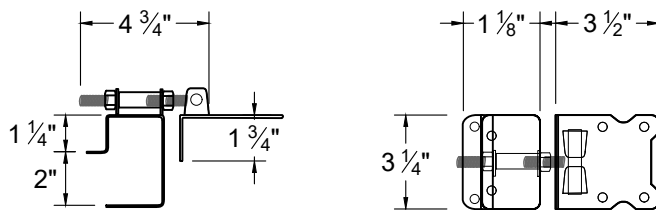
GATE HANDLE
