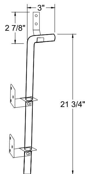
DROP ROD ASSEMBLY
