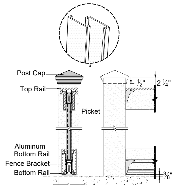
CUT VIEWS
