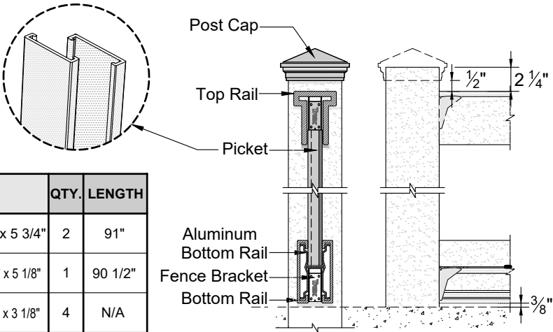
CUT VIEWS
