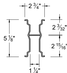
LENGTH: 90 1/2" (11 GA.)
