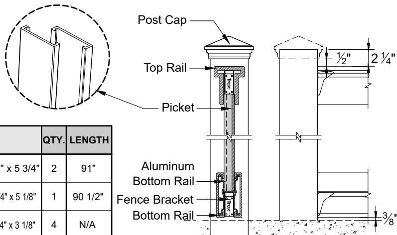
CUT VIEWS
