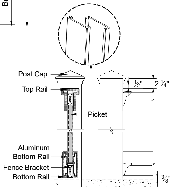
CUT VIEWS
